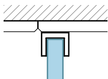
Wandprofil AP Profil mural apparent
